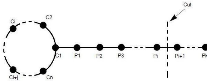
Figure 1: Tadpole graph in which the cut is done on the path graph
