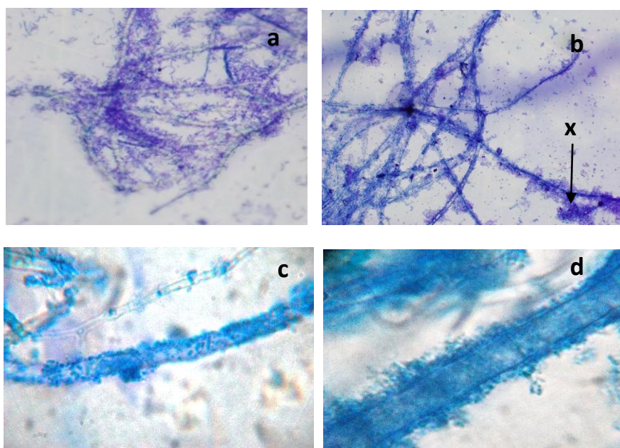
Figure 2: Bacterial colonization on A. niger mycelium in FBBs (a) colonization of B. subtilis , (b) P. aeruginosa , on A. niger mycelium in FBBs at x 400 magnification. (c) B. subtilis (d) P. aeruginosa , on A. niger mycelium in FBBs at x 1000 magnification. Darkness (x) is due to lactophenol cotton blue stain absorbed by EPS produced by the biofilms
