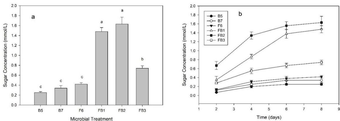
Figure 3: Cellulolytic activity in the form of sugar production by biofilms and their single cultures. Fig.3a shows sugar production after eight days of incubation. Fig.3b shows sugar production with the time. Columns with the same letter are not significantly different at 5% probability level. Vertical bars show standard deviations
