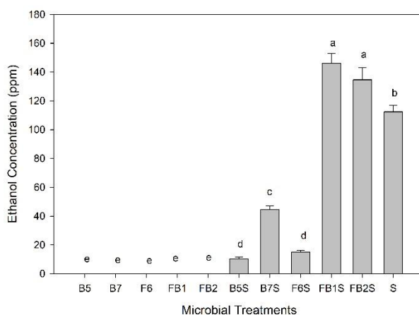
Figure 4: Ethanol production by different microbial treatments. B5, B7, F6, FB1 and FB2 are the treatments without co-culturing of S. cerevisiae . B5S, B7S, FB1S, FB2S are microbial treatments co-cultured with S. cerevisiae . S is only S. cerevisiae treatment. Columns with the same letter are not significantly different at 5% probability level. vertical bars show standard deviations
