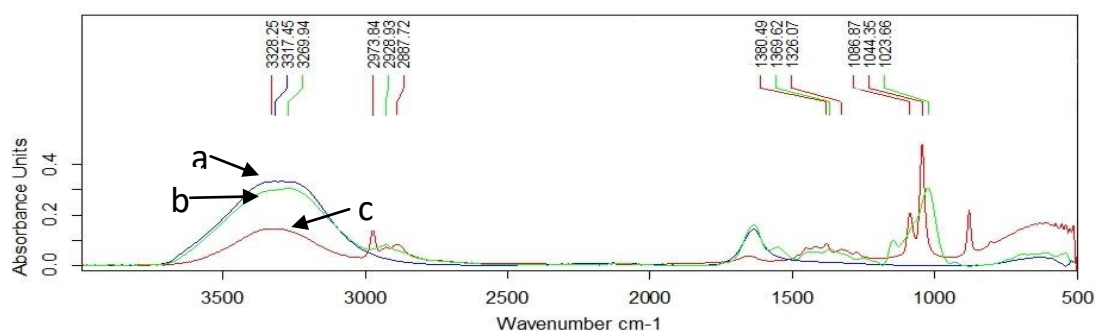
Figure 5: FTIR spectra for ethanol production by the responsive bio-films; (a) Bio-film FB1 with S. cerevisiae . (b) Bio-film FB2 with S. cerevisiae . (c) Pure ethanol.
