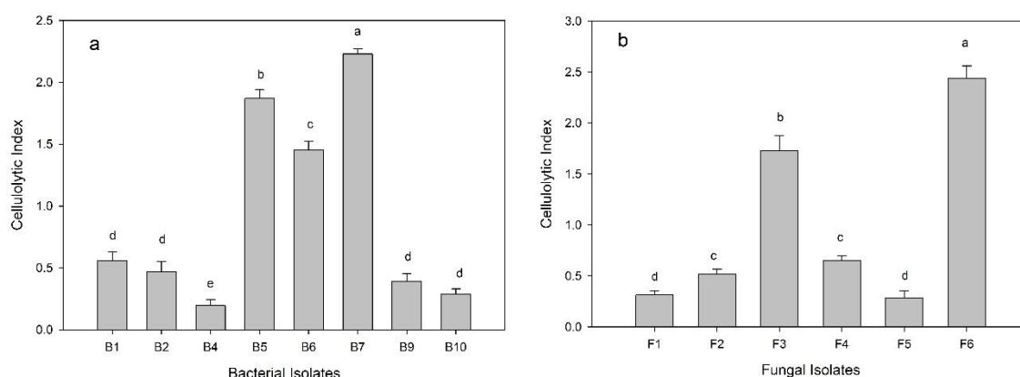
Figure 1: Cellulolytic index of isolated microorganisms (a) Bacterial cellulolytic index (b) fungal cellulolytic index. Columns with the same letter are not significantly different at 5% probability level. Vertical bars show standard deviations
